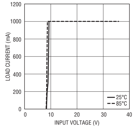
Minimum Required Input Voltage vs Output Load (8V OUT )
