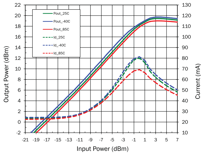
Output Power versus Input Power ( V_D = 3V , 900 MHz)
