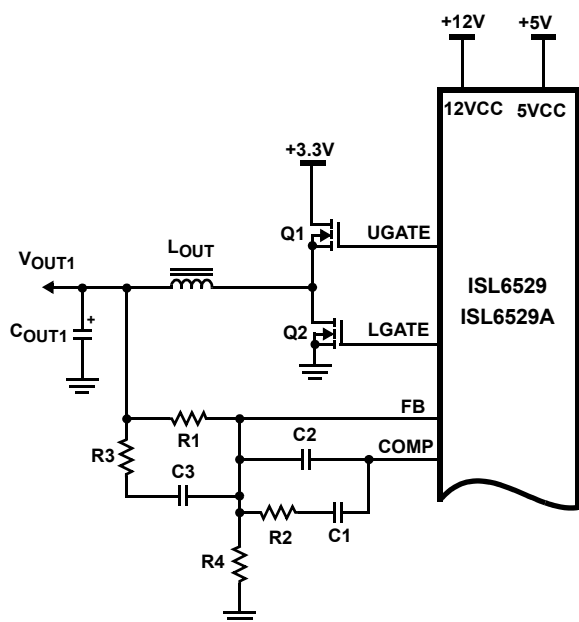
FIGURE 4. OUTPUT VOLTAGE SELECTION OF THE PWM
