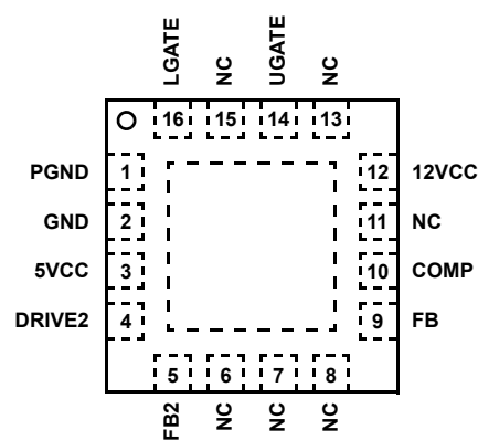
ISL6529, ISL6529A (QFN) TOP VIEW
