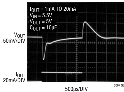
Transient Response
