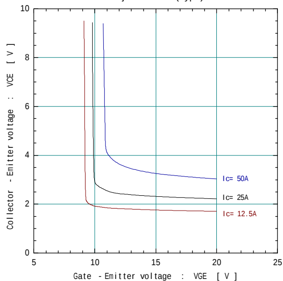
Collector-Emmitter voltage vs. Gate-Emmitter voltage Tj= 25 (typ.)
