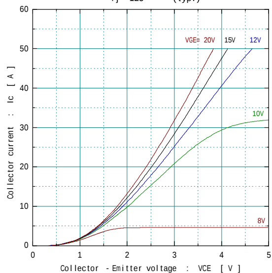
Collector current vs. Collector-Emmitter voltage Tj= 125 (typ.)
