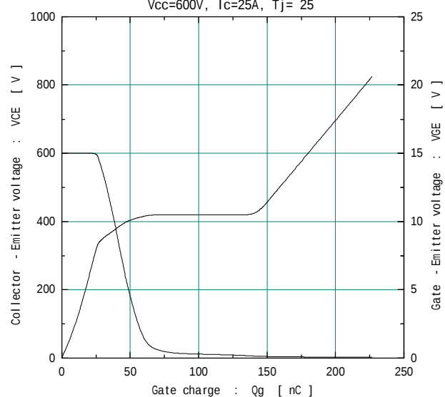
Dynamic Gate charge (typ.) Vcc=600V, Ic=25A, Tj= 25
