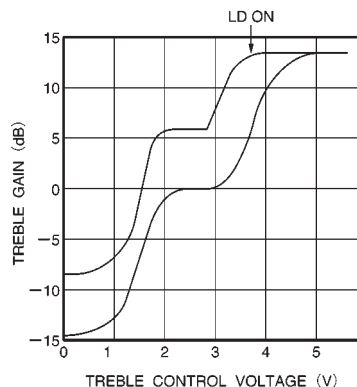
Fig.7 Treble gain vs. treble control voltage
