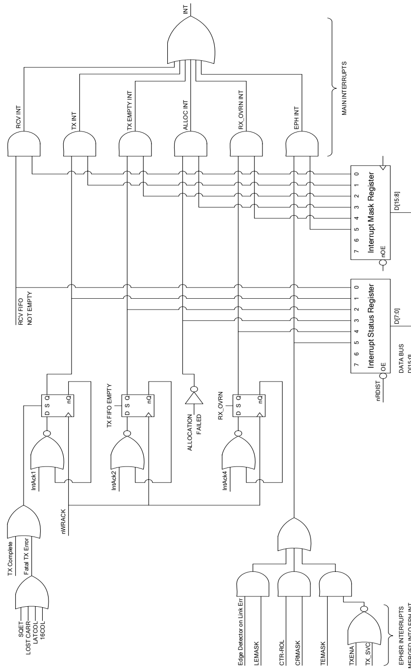
Figure 5.2 – Interrupt Structure
