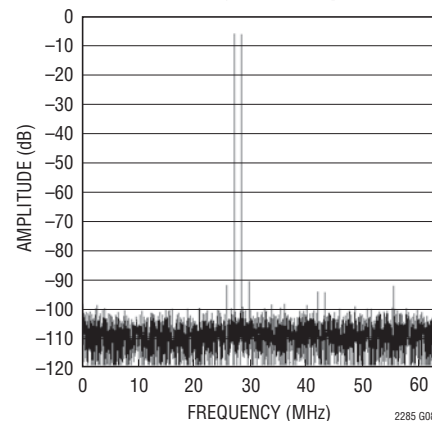
8192 Point 2-Tone FFT, f_{IN} = 28.2\text{MHz} and 26.8\text{MHz} , -1dB, 2V Range, 125Msps
