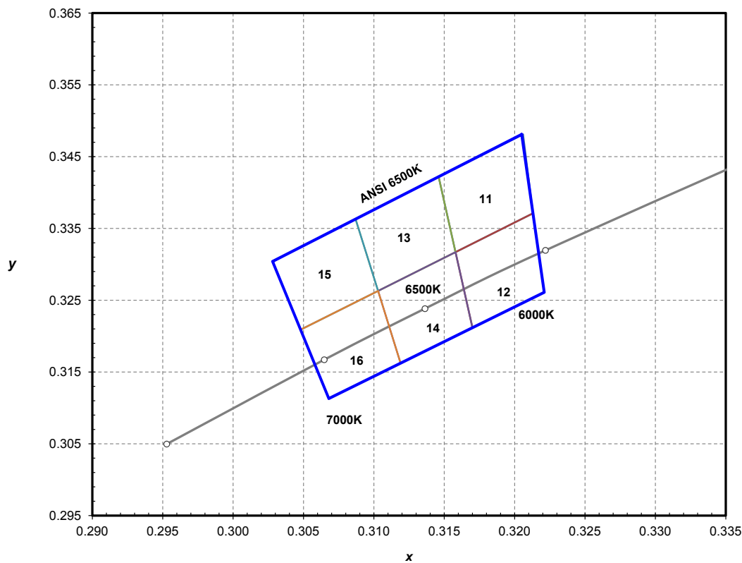
Figure 21. ANSI 6500K 1/6th color bin structure, forward current = 100 mA, thermal pad temperature = 25°C.
