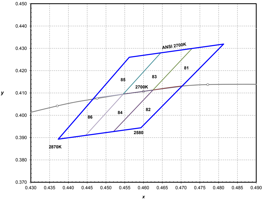
Figure 15. ANSI 2700K 1/6th color bin structure, forward current = 100 mA, thermal pad temperature = 25°C.
