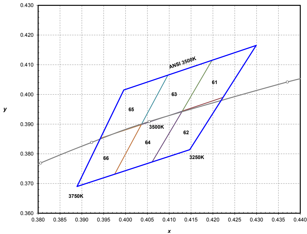
Figure 17. ANSI 3500K 1/6th color bin structure, forward current = 100 mA, thermal pad temperature = 25°C.
