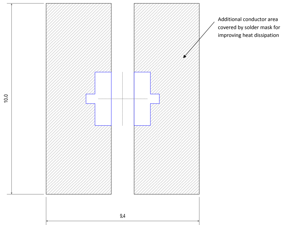
Figure 3. Solder pad layout.
