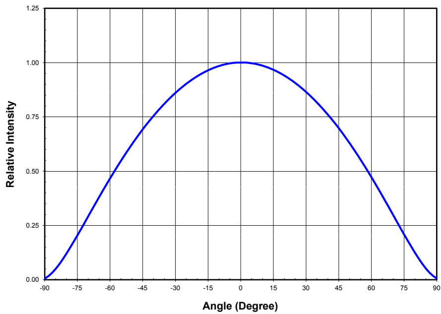
Figure 10. Typical representative spatial radiation pattern.
