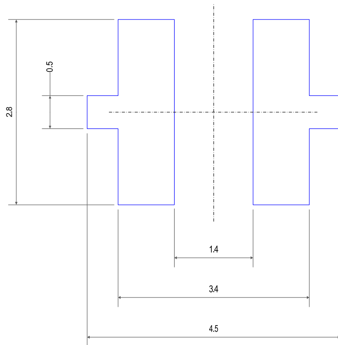
Recommended Pad Layout Dimensions
