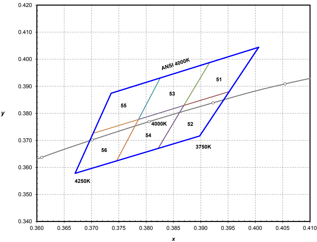
Figure 18. ANSI 4000K 1/6th color bin structure, forward current = 100 mA, thermal pad temperature = 25°C.
