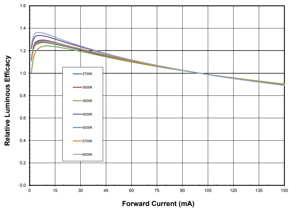
Figure 8. Typical emitter efficacy versus forward current, solder pad temperature = 25°C.
