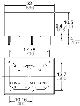
1 Form A type
