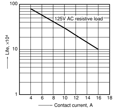
4. Life curve
