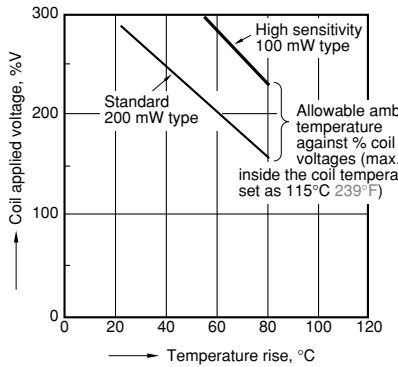
5.-(4) Ambient temperature characteristics (High sensitivity type) Contact current: 10 A
