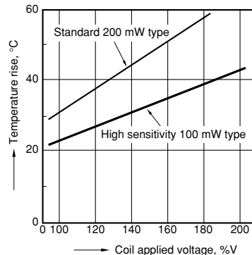
3.-(3) Coil temperature rise (High sensitivity type) Measured portion: Inside the coil
