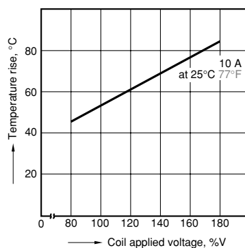
3.-(2) Coil temperature rise (1 Form C type) Measured portion: Inside the coil
