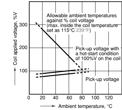
5.-(1) Ambient temperature characteristics (Standard 10 A type, 1 Form A) Contact current: 10 A
