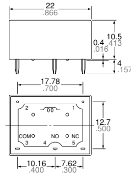
1 Form C type
