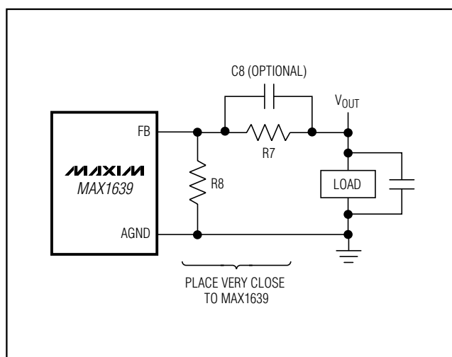
Figure 6. Output Selection
