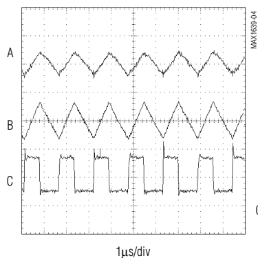
SWITCHING WAVEFORMS
