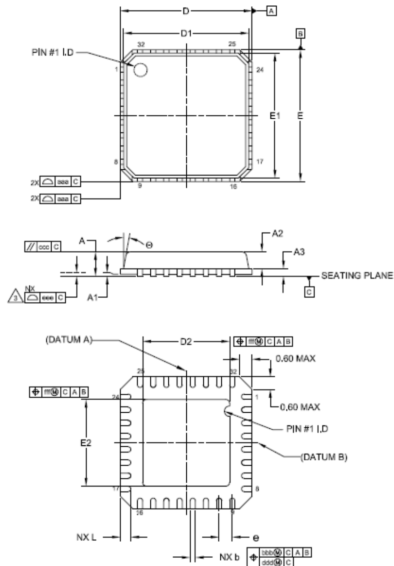
Figure 32. QFN32 - Outline
