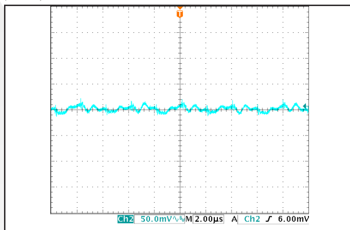
Figure 10: Output voltage ripple, V_{out} , at nominal input voltage and rated load current (50 mV/div). Load capacitance: 1μF ceramic capacitor and 10μF tantalum capacitor. Bandwidth: 10 MHz. See Figure 17.
