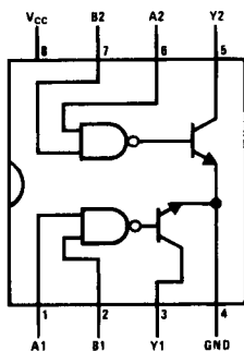
Top View Order Number DS55451J-8, DS75451M or DS75451N See NS Package Numbers J08A, M08A* or N08E
