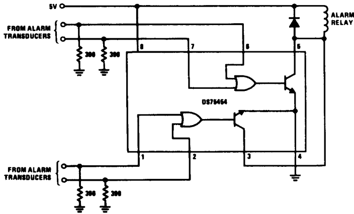
FIGURE 35. Alarm Detector
