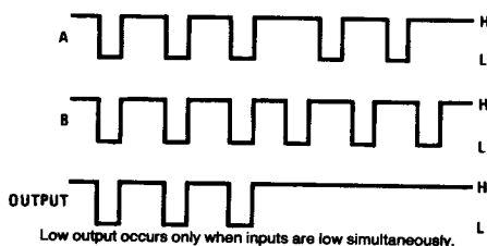
FIGURE 33. In-Phase Detector
