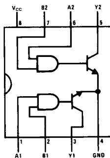
Top View Order Number DS55452J-8, DS75452M or DS75452N
