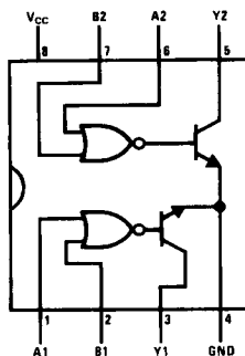
Top View Order Number DS55453J-8, DS75453M or DS75453N
