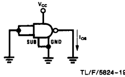
Each input is tested separately. FIGURE 5. I_{OS}
