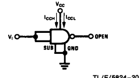
Both gates are tested simultaneously. FIGURE 6. I_{CCH} , I_{CCL}
