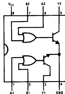
Top View Order Number DS55454J-8, DS75454M or DS75454N
