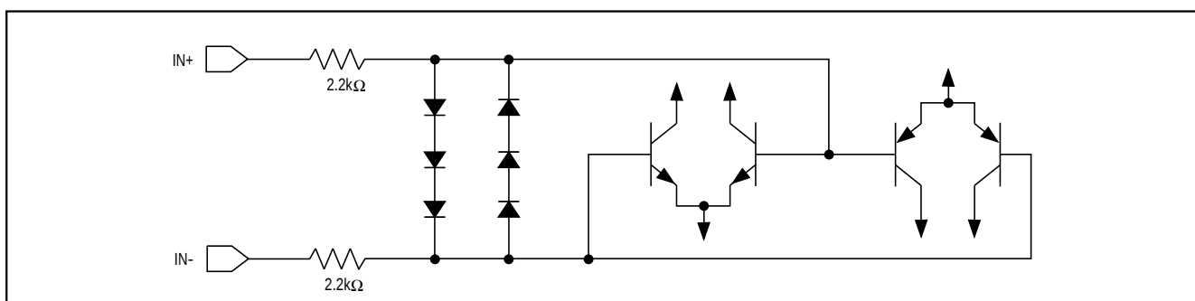
Figure 2. Input Protection Circuit
