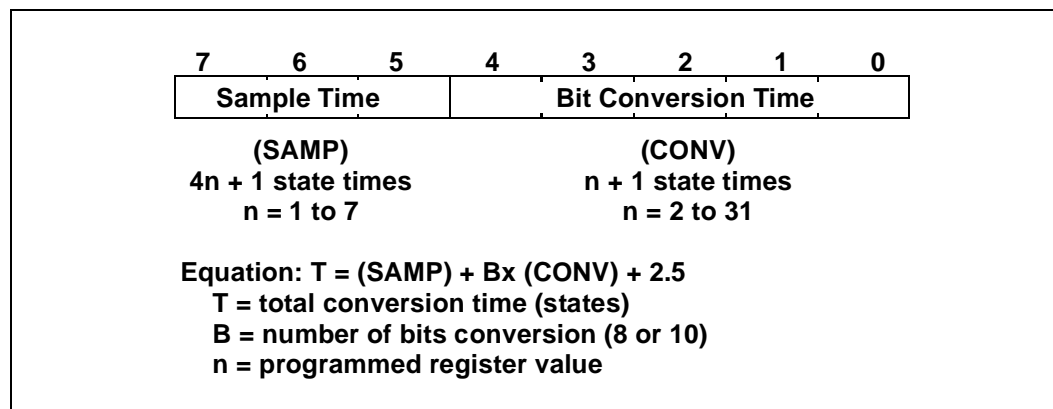
Figure 21. AD_TIME 1FAFH:Byte
