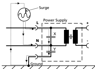
Fig. 23-5 Earthed input
