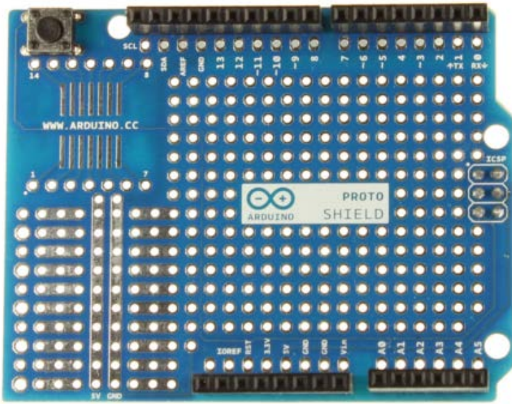
Proto Shield R3 mounted Front
