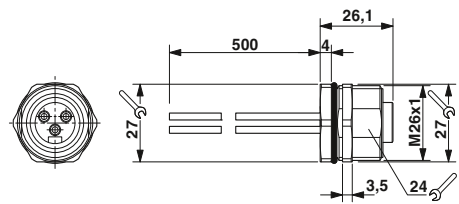
7/8" flush-type socket
