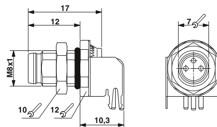
M8 flush-type plug, angled
