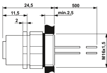
M12 flush-type socket, can be positioned
