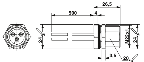
7/8" flush-type plug
