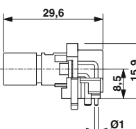
M12 pin contact carrier, angled, 4, 5-pos.
