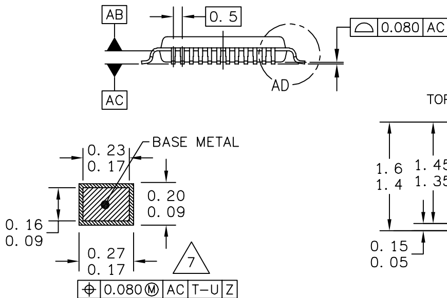
SECTION AE-AE
