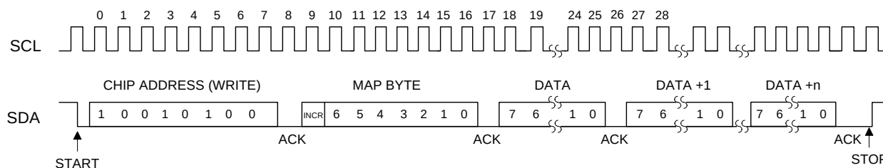
Figure 20. Control Port Timing, I 2 C Write
