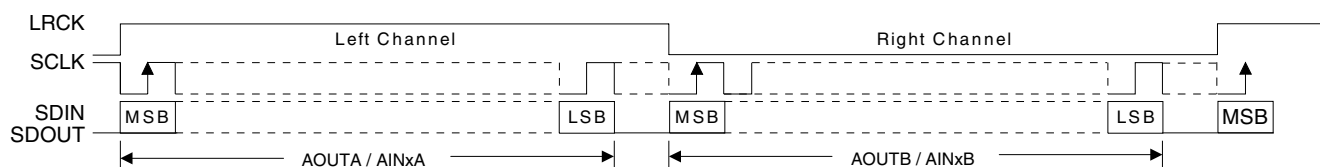
Figure 17. Left-Justified Format
