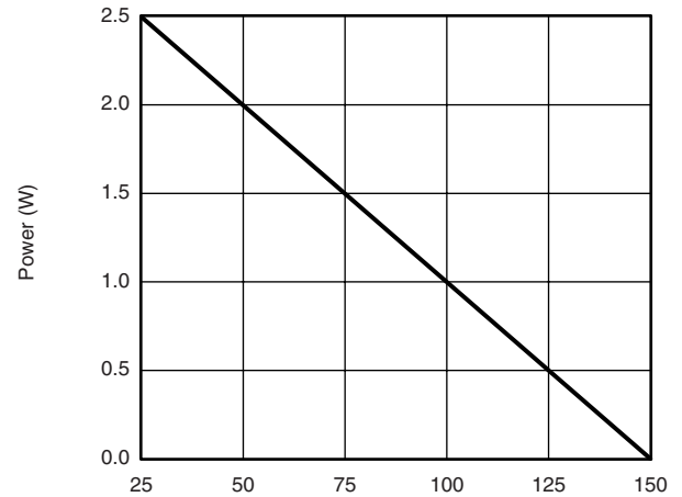
Power Derating
