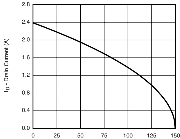
Current Derating*
