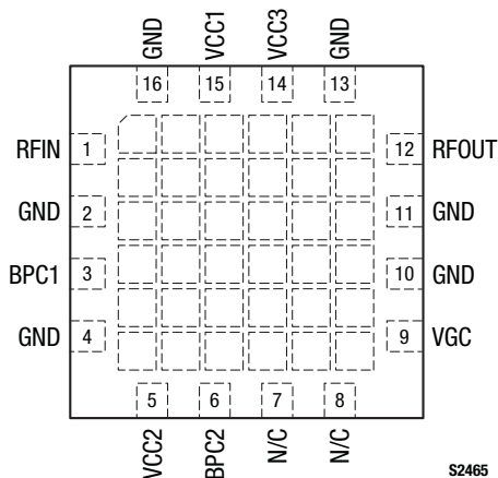
Figure 2. SKY65371-11 Pinout – 16-Pin MCM (Top View)
