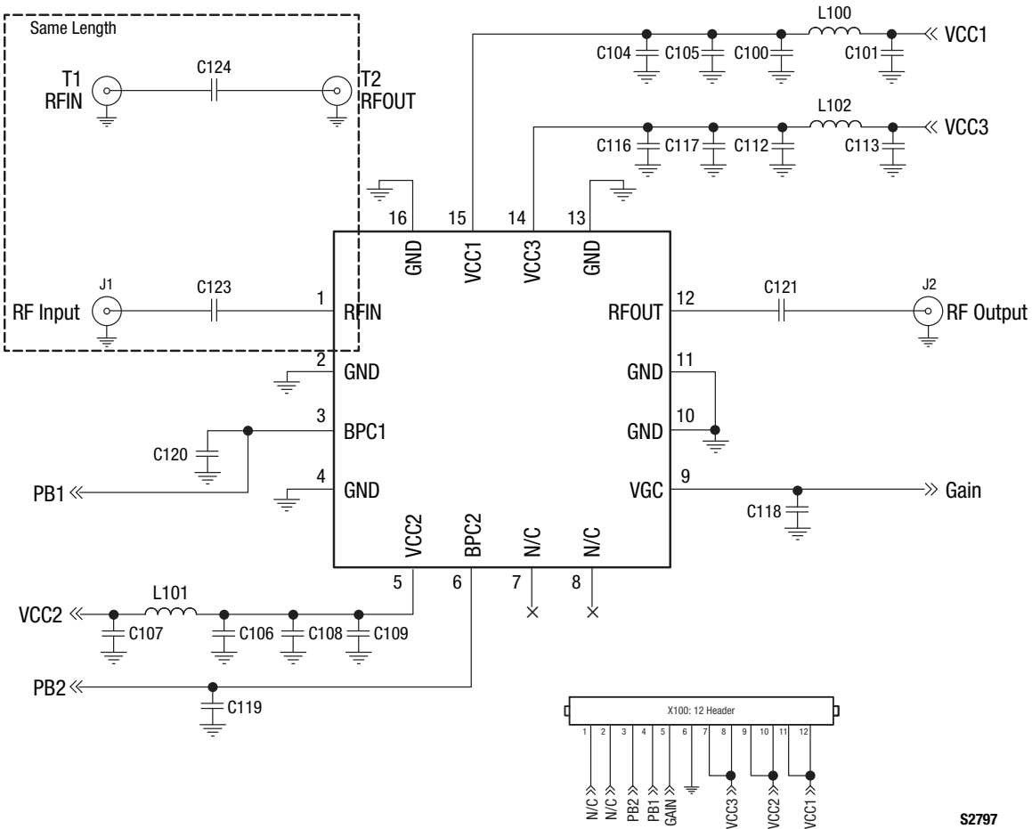
Figure 6. SKY65371-11 Evaluation Board Schematic
