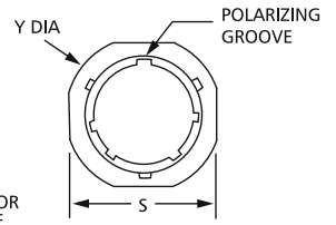
RECEPTACLE ASSEMBLY
