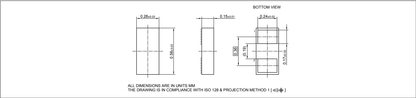
Figure 12 WLL-2-3 package outline (dimension in mm)
