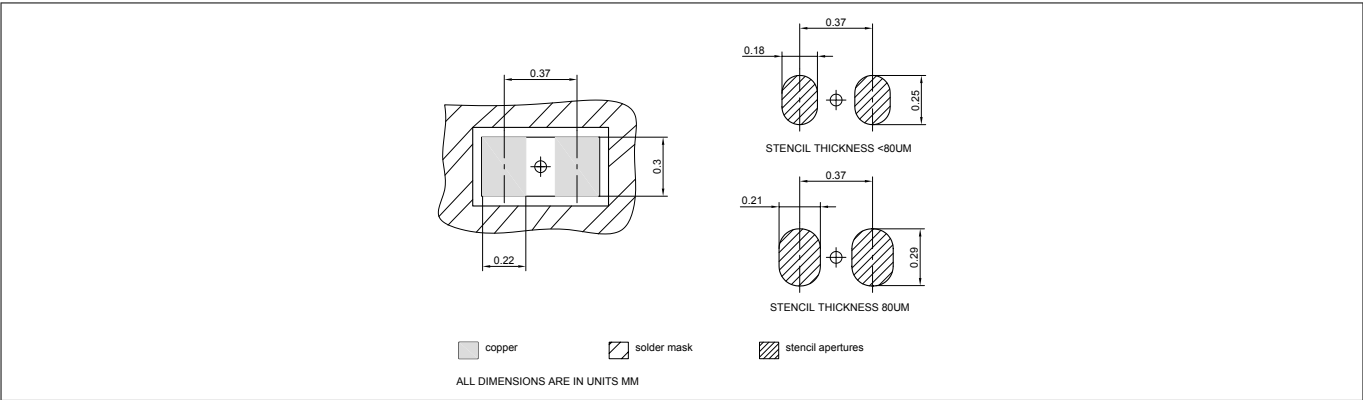
Figure 13 WLL-2-3 footprint (dimension in mm), recommendation for Printed Circuit Board Assembly see [2]
