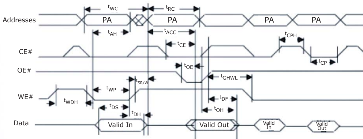
Figure 15.7 Back to Back Read/Write Cycle Timing
