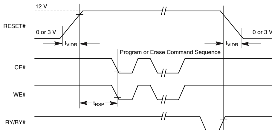
Figure 15.12 Sector Protect/Unprotect Timing Diagram
