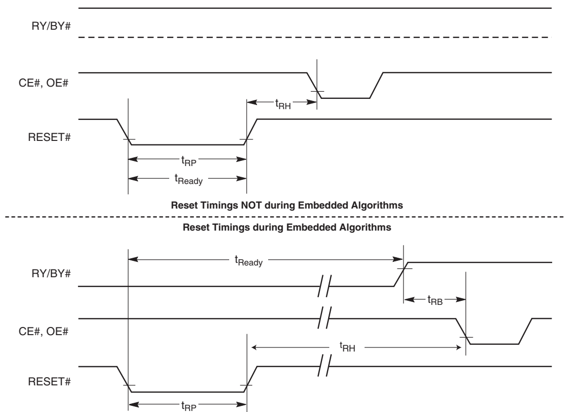
Figure 15.2 RESET# Timings
