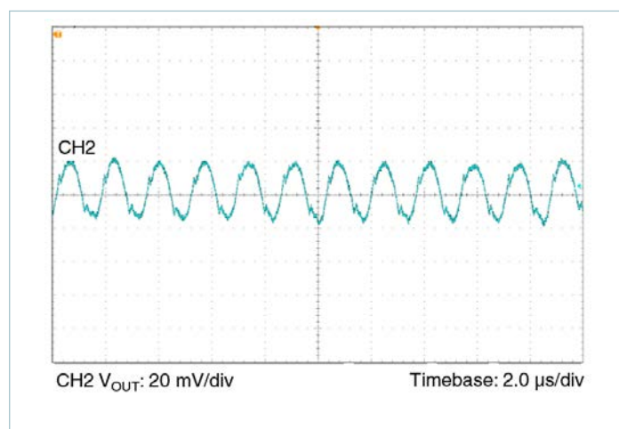
Figure 29 — Output Ripple 12 V IN 5.0 V OUT at 15 A; C_{OUT} = 8 x 47 \mu F
