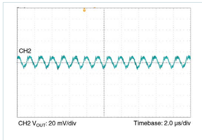
Figure 30 — Output Ripple 12 V IN 5.0 V OUT at 7.0 A; C_{OUT} = 8 x 47 \mu F
