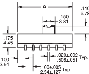
L Type Surface Mount
