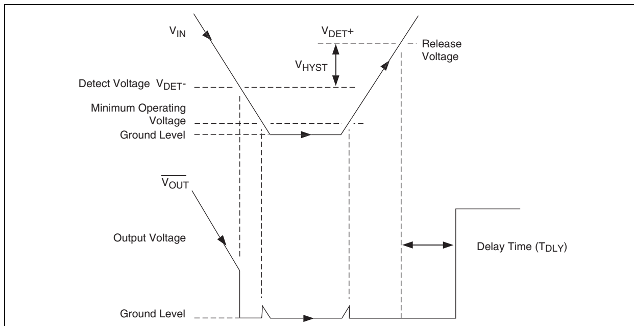
FIGURE 3-1: TIMING DIAGRAM
