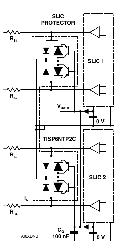
Figure 2. SLIC Protection
