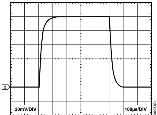
Figure 29. Small Signal Pulse Response, G = 1000 , R_L = 25 kΩ, C_L = 100 pF
