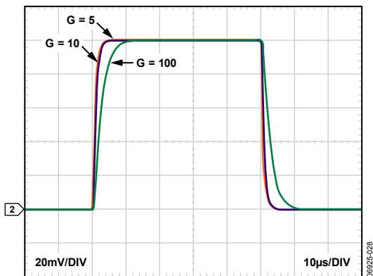
Figure 28. Small Signal Pulse Response, G = 5, 10, 100 ; R_L = 10 kΩ
