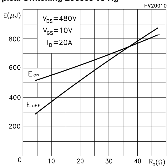
Typical Switching Losses vs Rg
