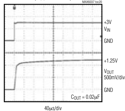
MAX6037_12 TURN-ON TRANSIENT ( V_{OUT} = 1.25V )
