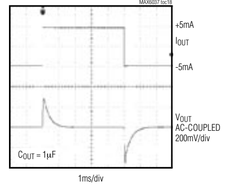
MAX6037_41 LOAD TRANSIENT ( V_{OUT} = 4.096V )
