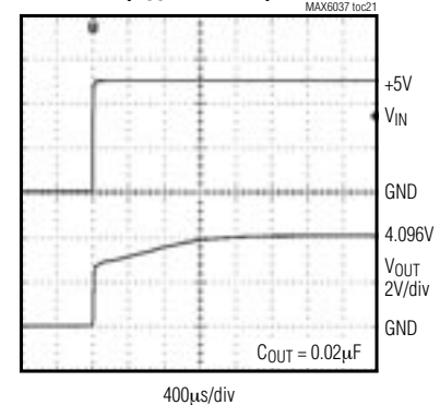
MAX6037_41 TURN-ON TRANSIENT ( V_{OUT} = 4.096V )
