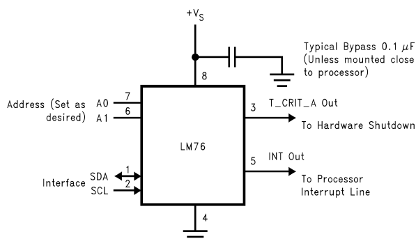
Figure 2. Typical Application
