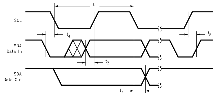
Figure 3. Timing Diagram
