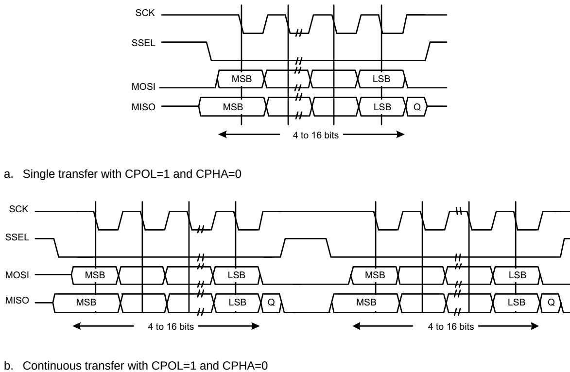
Fig 48. SPI frame format with CPOL = 1 and CPHA = 0 (a) Single and b) Continuous Transfer)
