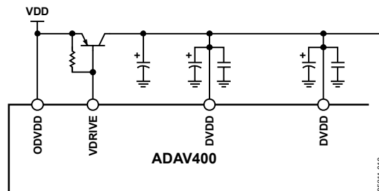
Figure 19. Voltage Regulator Design
