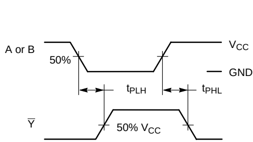
Figure 4. Switching Waveforms
