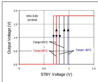
Fig 60. STBY Threshold
