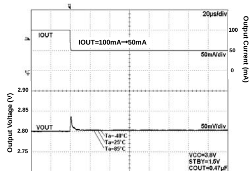
Fig 200. Load Response
