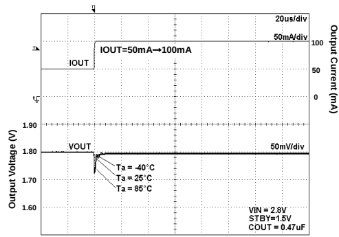
Fig 70. Load Response
