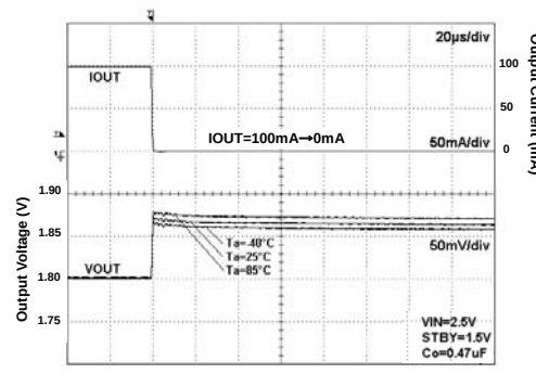
Fig 67. Load Response
