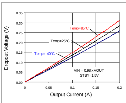
Fig 135. Dropout Voltage
