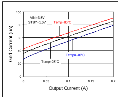
Fig 107. IOUT - IGND
