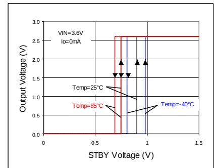
Fig 137. STBY Threshold
