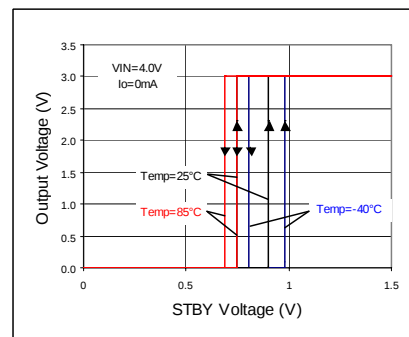
Fig 215. STBY Threshold
