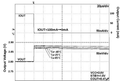
Fig 196. Load Response
