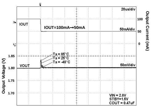
Fig 71. Load Response
