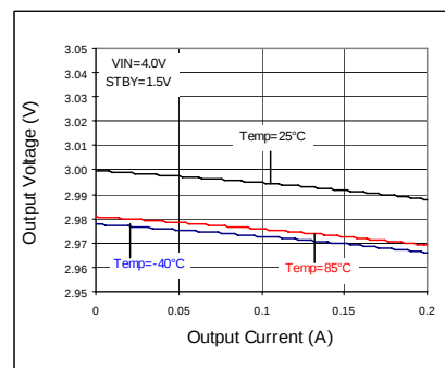
Fig 212. Load Regulation
