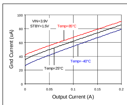
Fig 82. IOU - IGND
