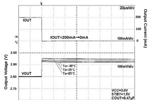
Fig 198. Load Response
