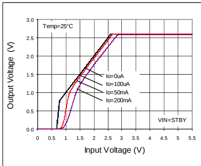
Fig 129. Output Voltage
