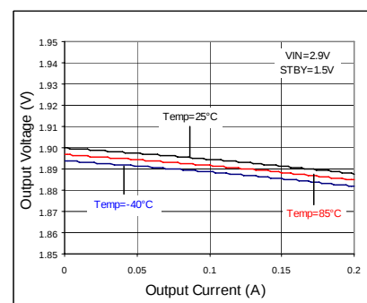
Fig 83. Load Regulation
