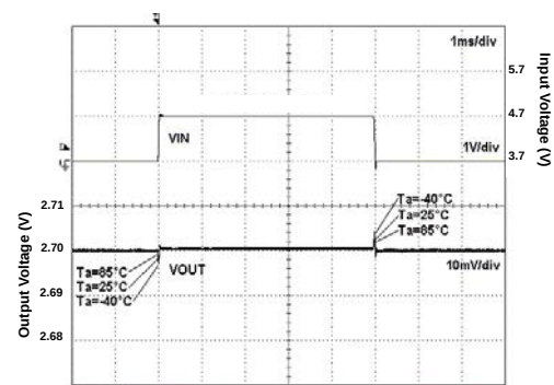
Fig 180. VIN Response
