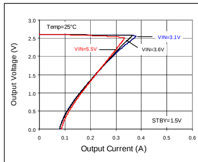
Fig 136. OCP Threshold
