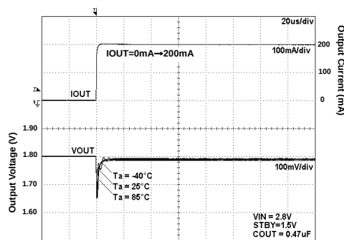
Fig 68. Load Response
