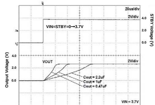
Fig 178. Start Up Time (VIN=STBY) Iout=200mA
