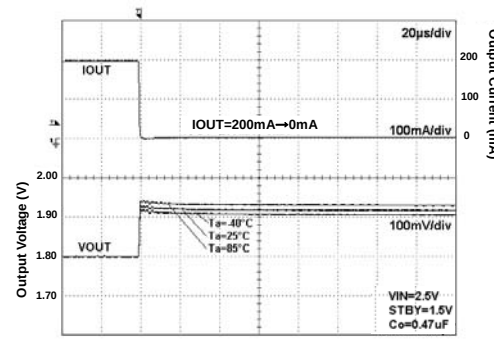
Fig 69. Load Response
