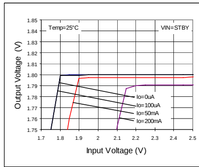
Fig 54. Line Regulation
