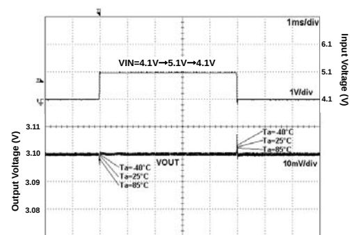
Fig 258. VIN Response
