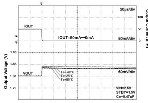
Fig 65. Load Response
