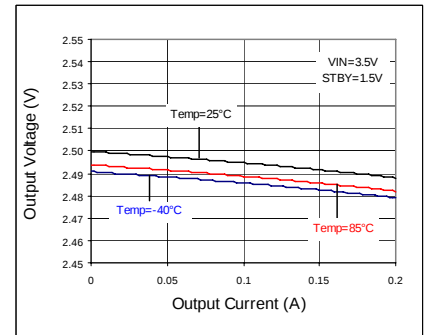
Fig 108. Load Regulation
