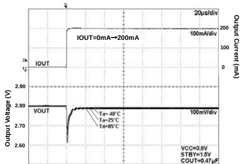
Fig 197. Load Response
