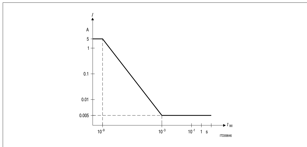
Figure 89 U-Transceiver Input Current
