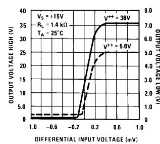
Transfer Function
