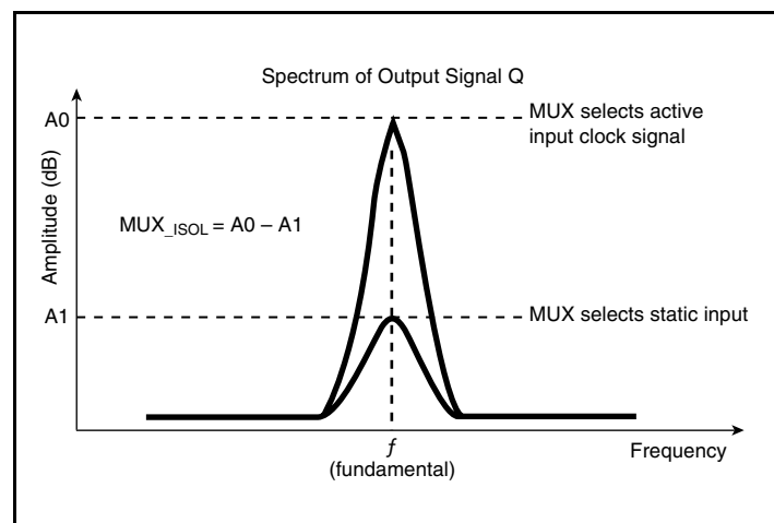
MUX_ISOLATION
