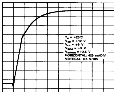
Figure 9. Positive-Going Settling Time
