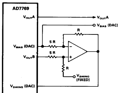
Figure 28. Generating a Software Programmable V_{SWING} (DAC)
