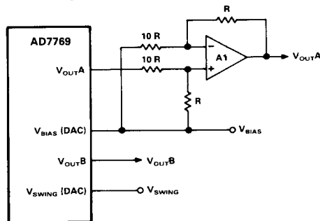
Figure 25. Increasing the DAC Output Voltage Resolution
