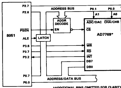
Figure 20. AD7769 to 8051 (Processor Bus) Interface
