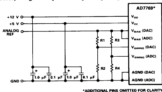
Figure 7. Typical Analog Connections to the AD7769
