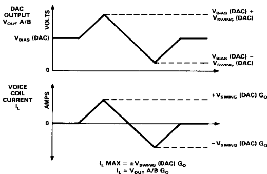
Figure 24. Typical Relationship Between Input Voltage and Output Current for Transconductance Amplifier
