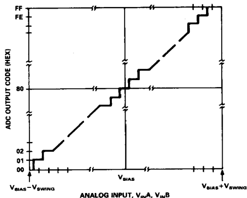
Figure 5. ADC Transfer Function
