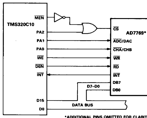
Figure 18. AD7769 to TMS320C10 Interface
