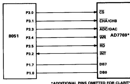
Figure 21. AD7769 to 8051 (Parallel I/O Ports) Interface
