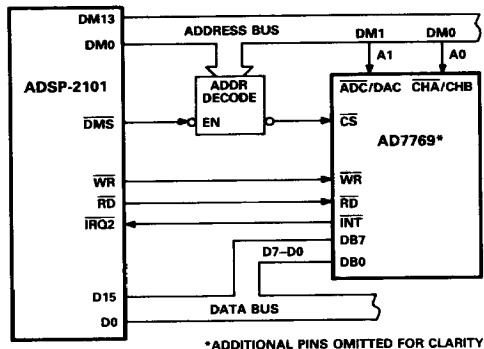
Figure 19. AD7769 to ADSP-2101 Interface
