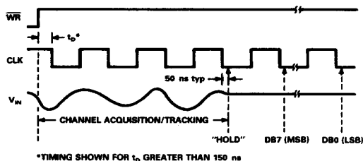
Figure 8. Operating Waveforms Using External Clock
