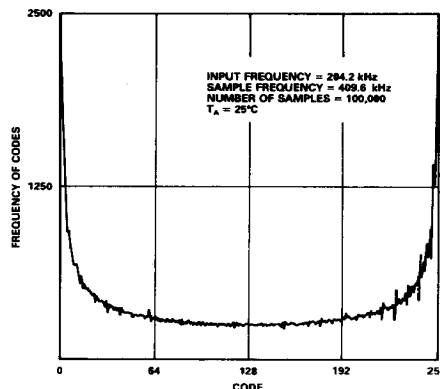
Figure 17. ADC Histogram Plot
