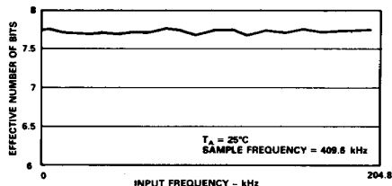
Figure 15. Effective Number of Bits vs. Frequency
