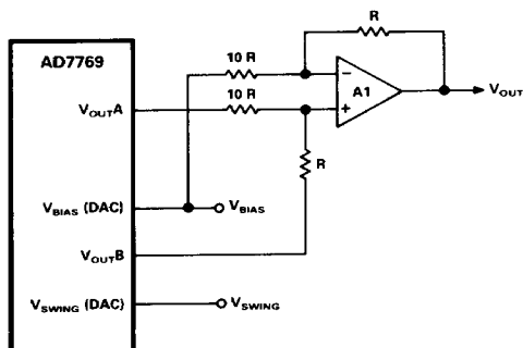
Figure 26. Combined V_{OUTA} , V_{OUTB} Circuit
