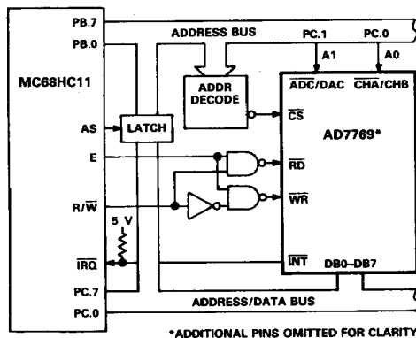
Figure 22. AD7769 to MC68HC11 Interfaced
