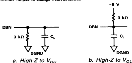
Figure 1. Load Circuits for Data Access Time Test
