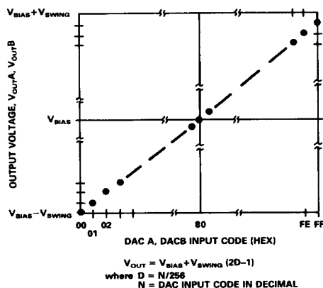
Figure 6. DAC Transfer Function
