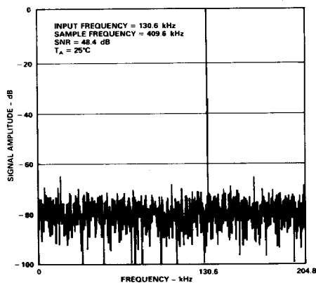
Figure 14. ADC FFT Plot
