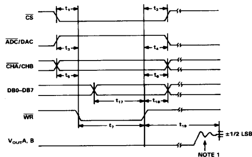
Figure 13. Timing for DAC Channel Select and Data Write
