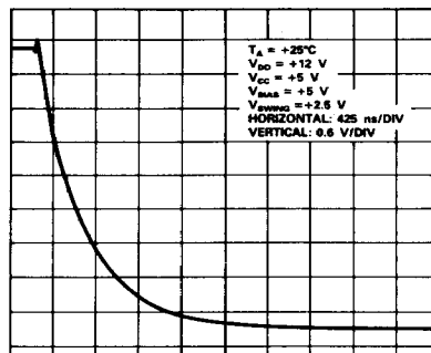
Figure 10. Negative-Going Settling Time
