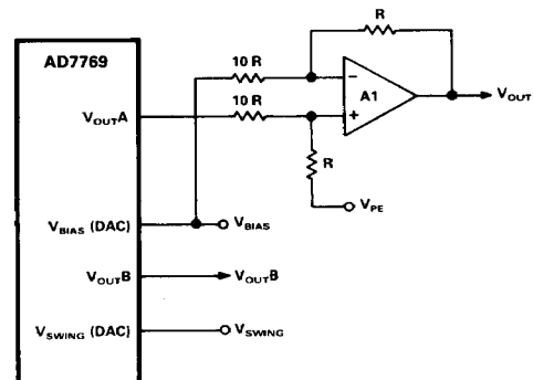
Figure 27. Servo Offset Facility
