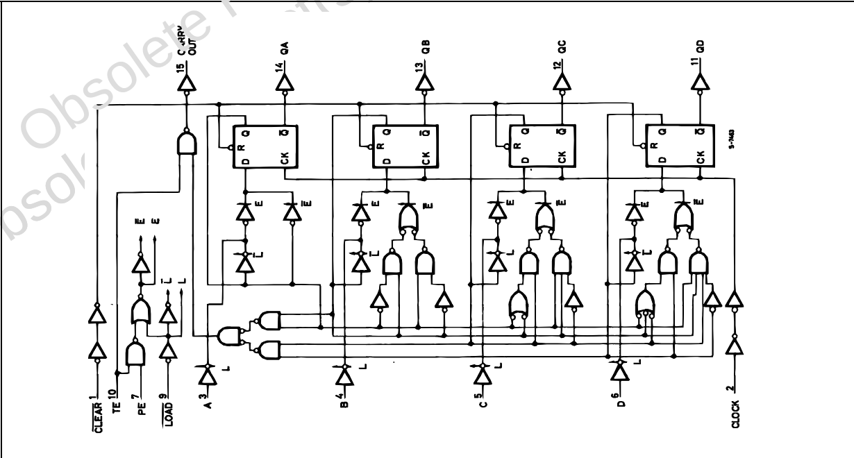
Figure 3: Logic Diagram
