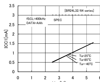
Fig.10 Current consumption at WRITE action ICC1 (fSCL=400kHz)
