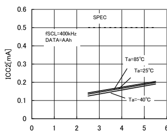
Fig.11 Current consumption at READ action ICC2 (fSCL=400kHz)
