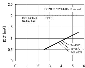
Fig.9 Current consumption at WRITE action ICC1 (fSCL=400kHz)
