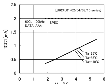
Fig.12 Current consumption at WRITE action ICC1 (fSCL=100kHz)
