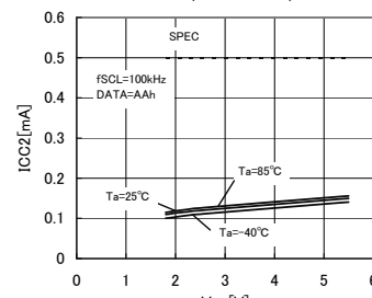
Fig.14 Current consumption at READ action ICC2 (fSCL=100kHz)
