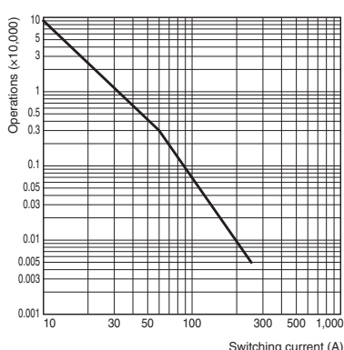
Electrical Endurance (Switching Performance)
