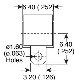
Solder Terminal
