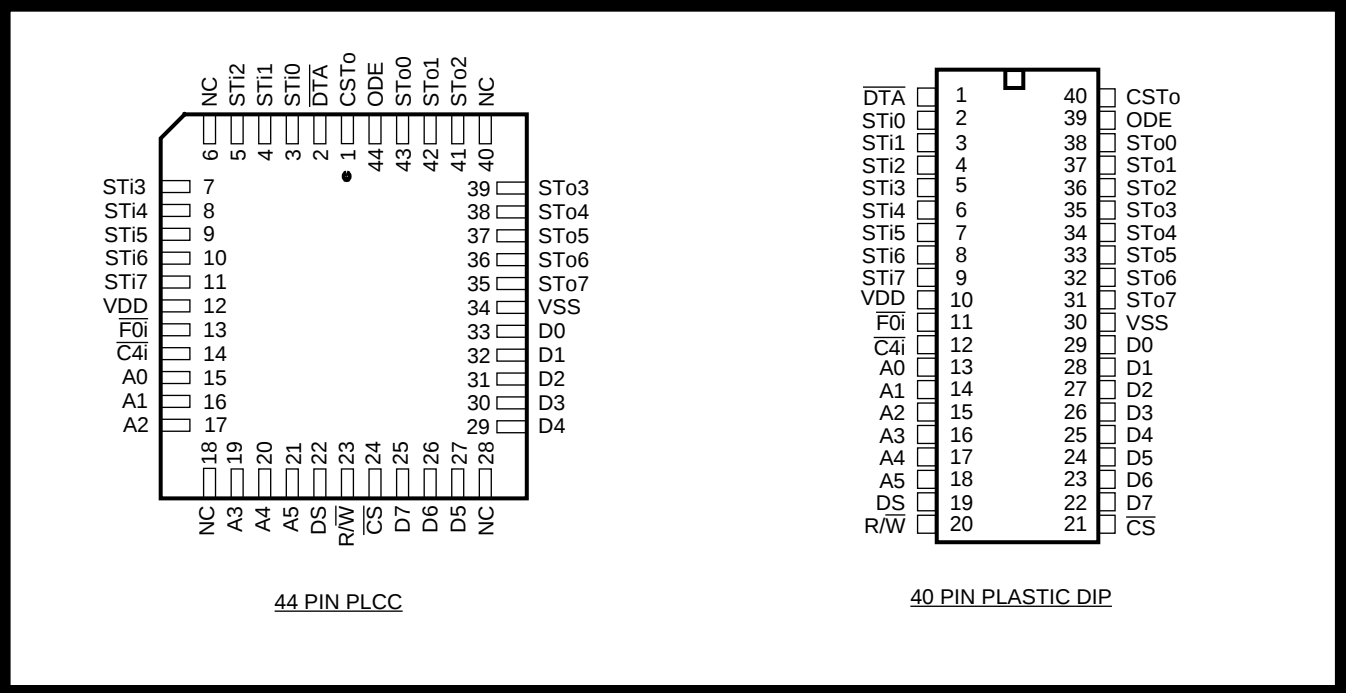
Figure 2 - Pin Connections
