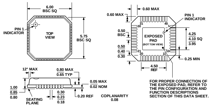
COMPLIANT TO JEDEC STANDARDS MO-220-VJJD-2 Figure 57. 40-Lead Lead Frame Chip Scale Package [LFCSP_VQ] 6 mm × 6 mm Body, Very Thin Quad (CP-40-1) Dimensions shown in millimeters
