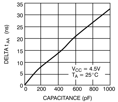
TYPICAL ACCESS TIME CHANGE vs. OUTPUT LOADING
