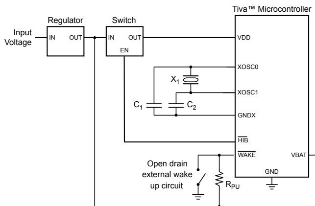
Figure 7-4. Using a Regulator for Both V_{DD} and V_{BAT}
